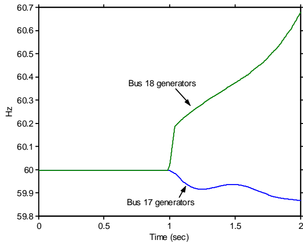
Fig. 8: Generator electrical speeds with the system operated at baseline loading with no load control for example 3.
